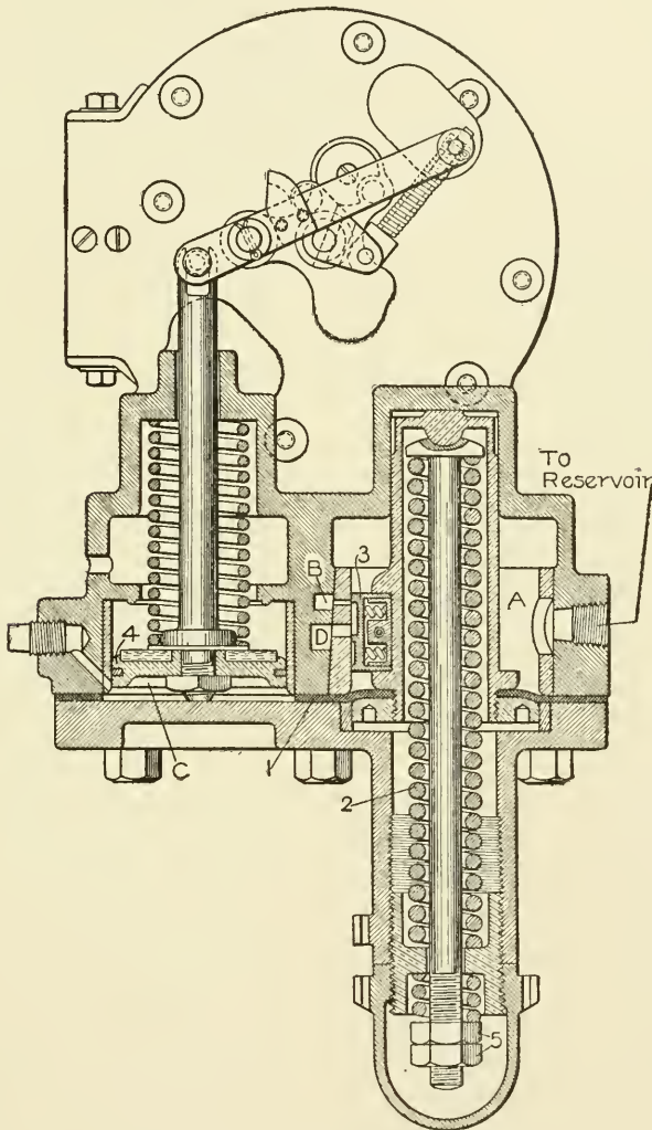
Fig. 90. Part Section of Pump Governor
